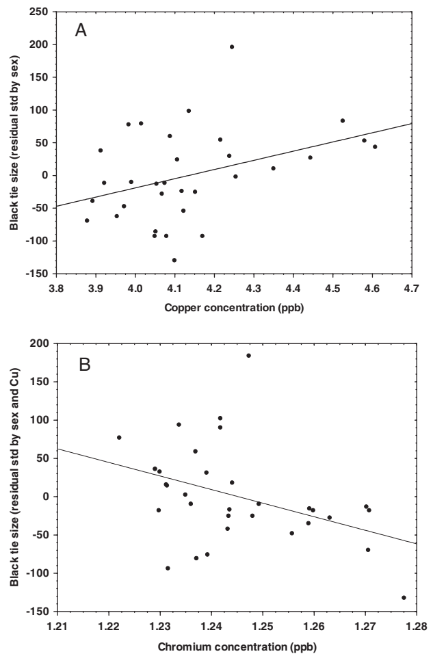
Fig. 1. Relationships between the feather (A) copper and (B) chromium concentrations and the size of the black tie. Residuals are presented to account for the effect of sex (A) and sex and copper levels (B) on tie size.
