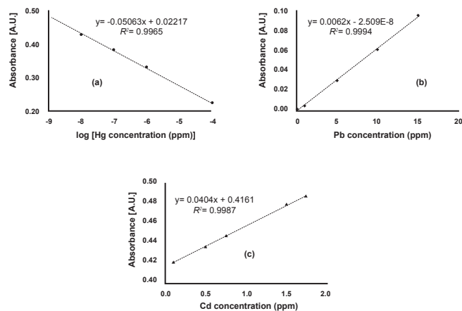
Fig. 2. Calibration curves for (a) Hg, (b) Pb, and (c) Cd used during this study.
